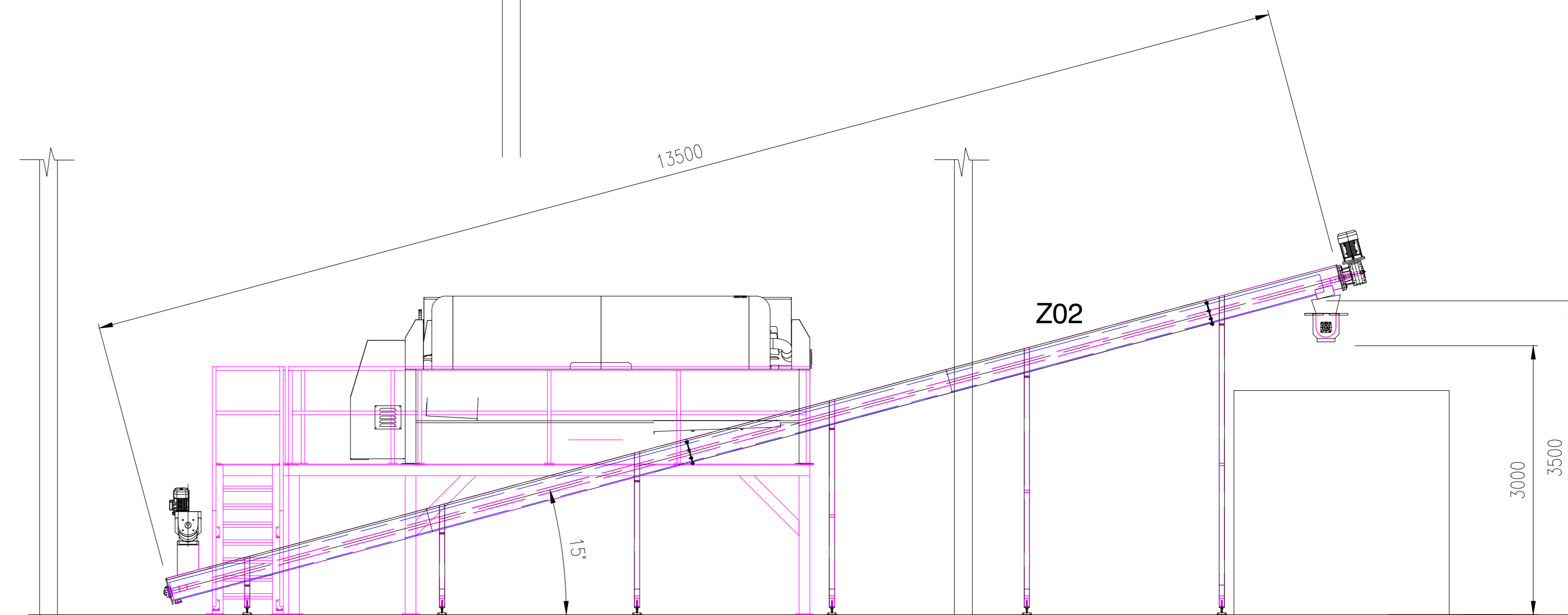
VIEW B-B
